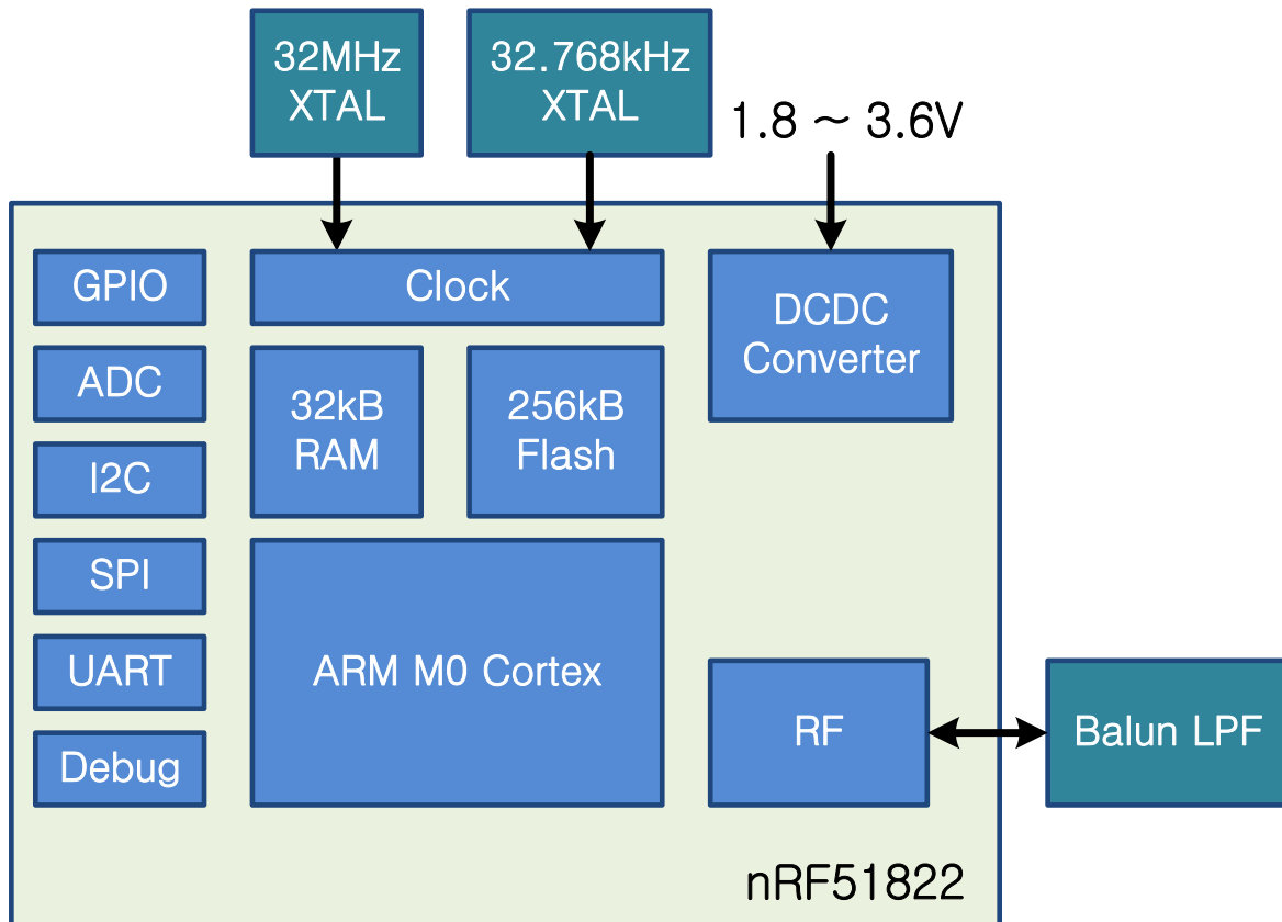
<Figure 2. Simplified block diagram of UTO-NBL-51M>
